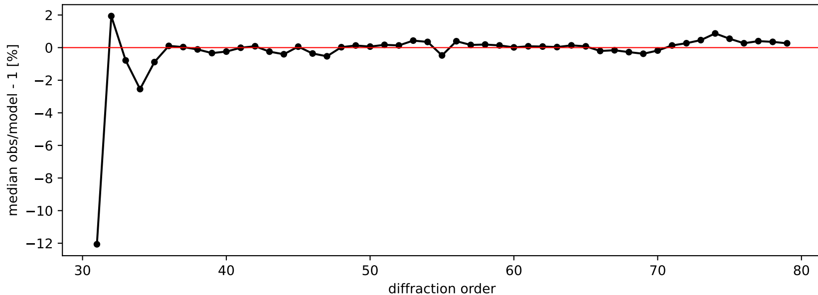
median offset per order, transmission: degree 1 spline
