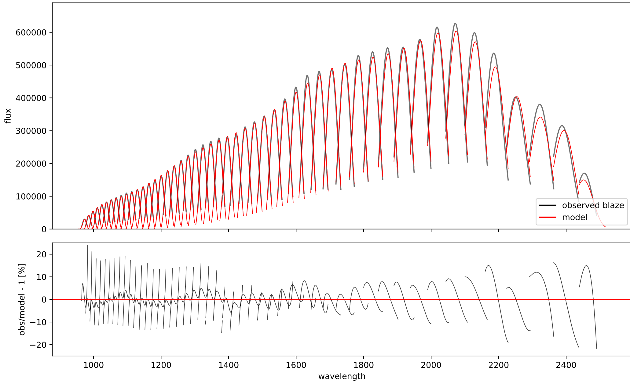
5000 K blackbody \times \exp(P_{11}) transmission \times \text{sinc}^2 blaze \times d\lambda/d\text{pix}
