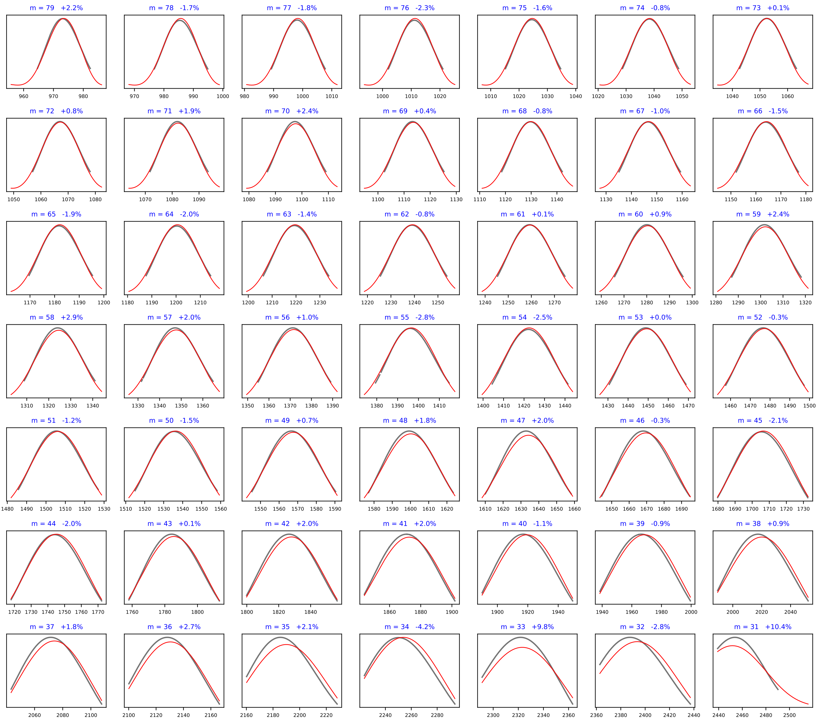
observed (black) vs model (red), median offset per order
