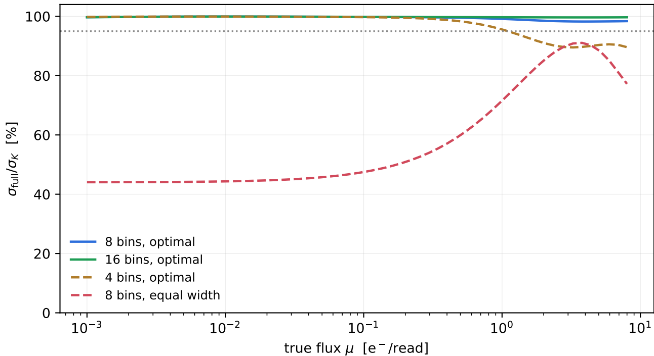
accuracy retained, across the whole flux range
