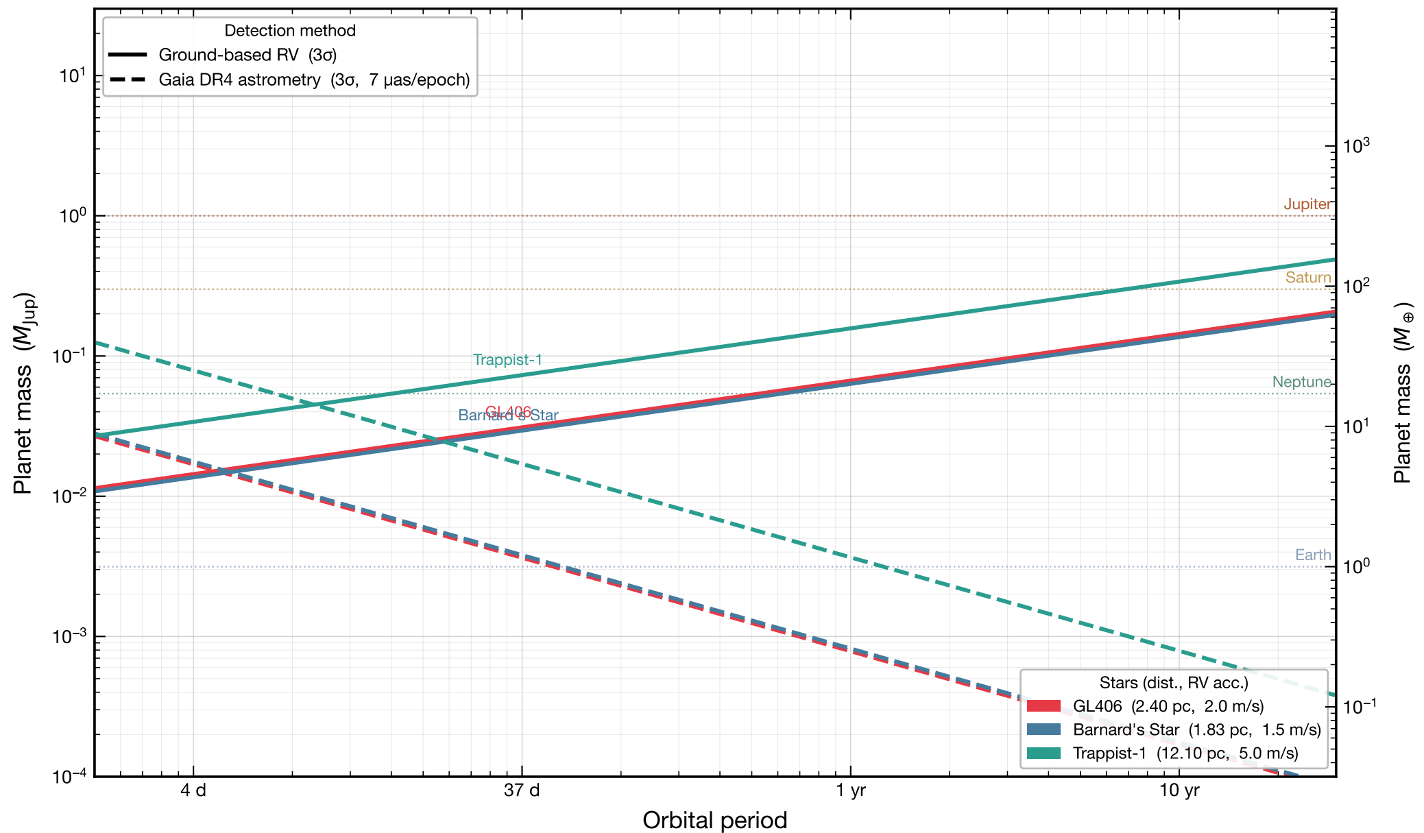
Planet detection limits: ground-based RV vs. Gaia DR4 astrometry (solid = RV, dashed = Gaia DR4 astrometry, 3\sigma threshold)
