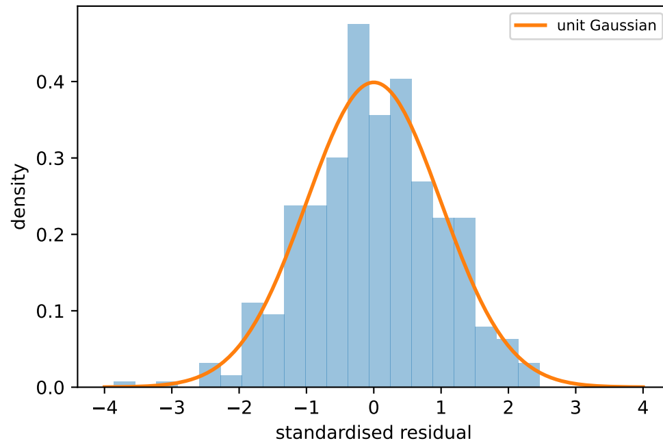
Band coverage
