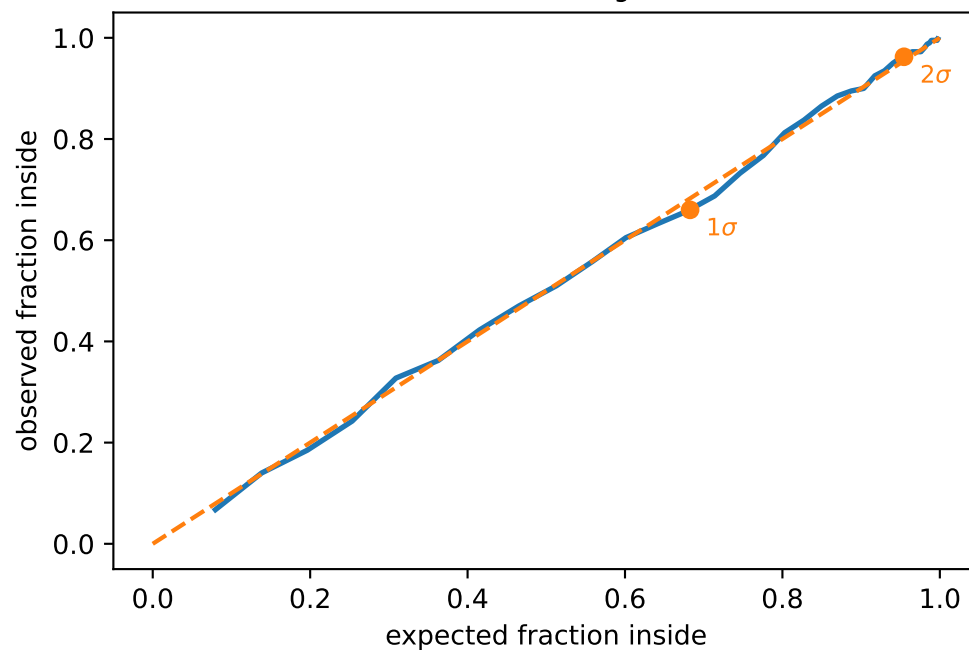
Band coverage
