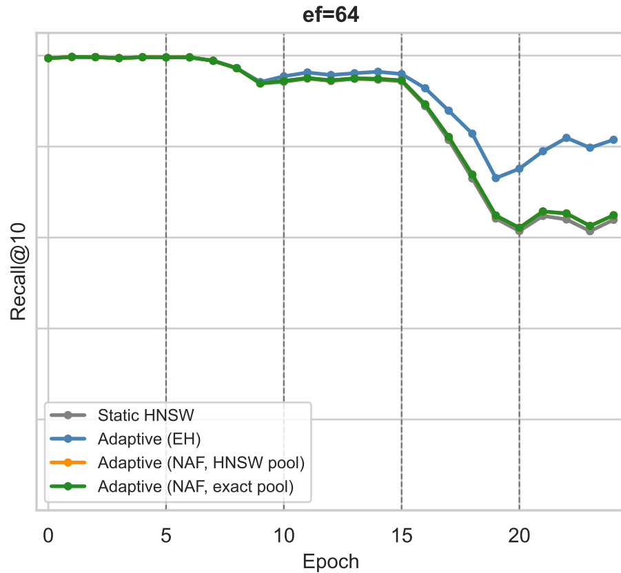
Recall@10 vs Epoch — NAF vs EH vs Static
