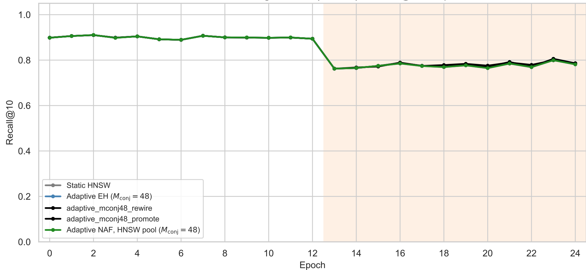
DEEP-96 cluster-reweighted drift (sudden) — recall@10 vs epoch
