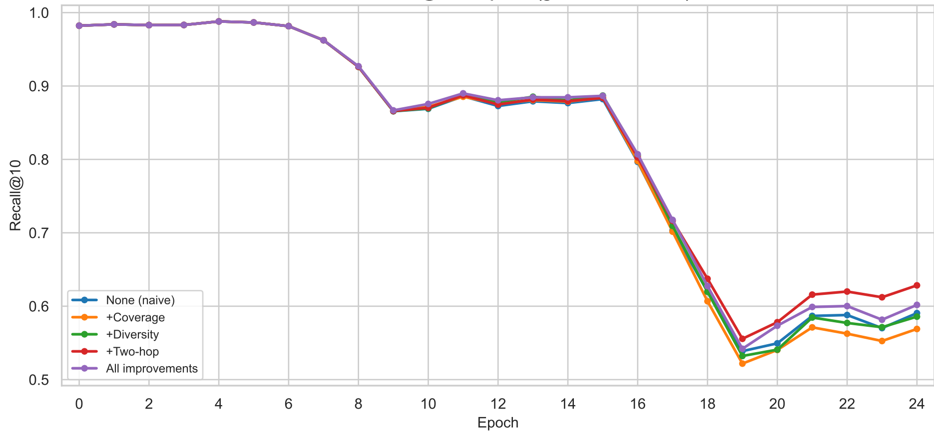
Ablation: recall@10 vs epoch (gradual drift, ef=32)
