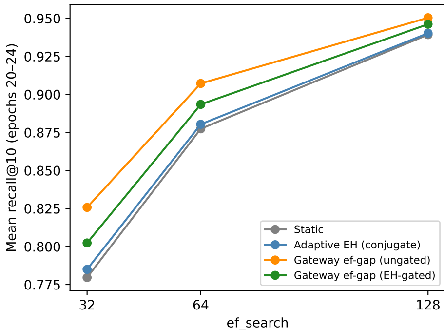
Ef-scaling at full drift — sudden
