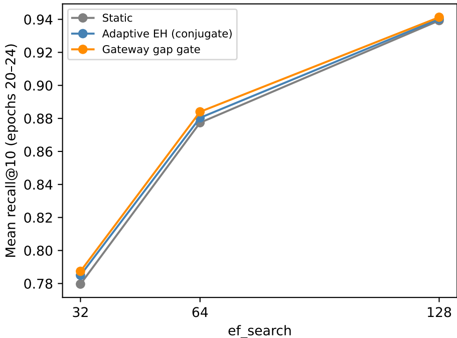
Ef-scaling at full drift — sudden
