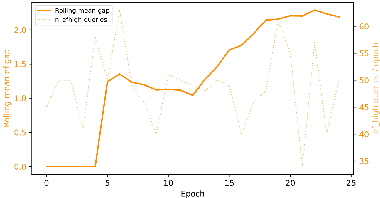
Gap signal and ef_high trigger rate — sudden drift
