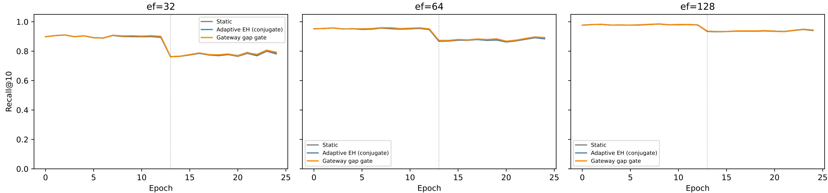
Recall@10 — sudden drift (DEEP-96 cluster, exp47)
