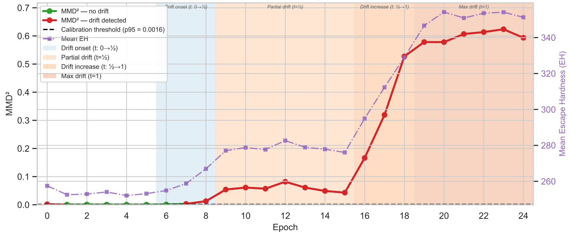
Drift Detector Signal Over Time (Gradual schedule)
