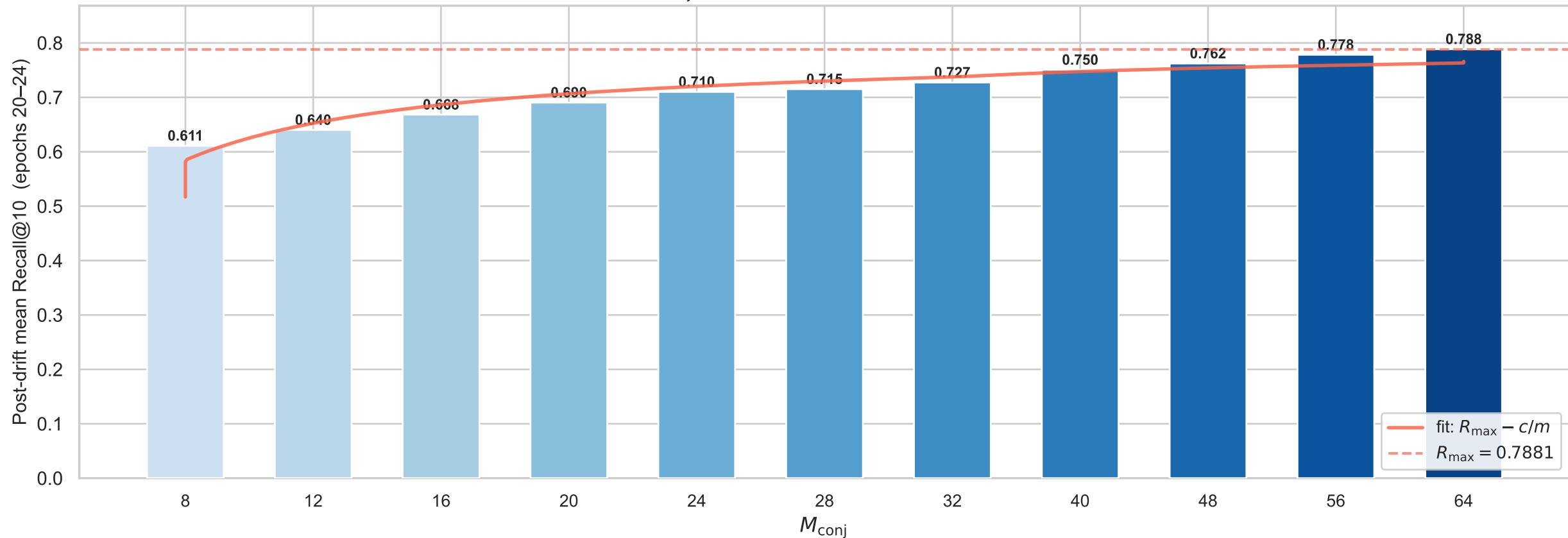
Full M_{\text{conj}} progression (gradual drift, ef=32)
