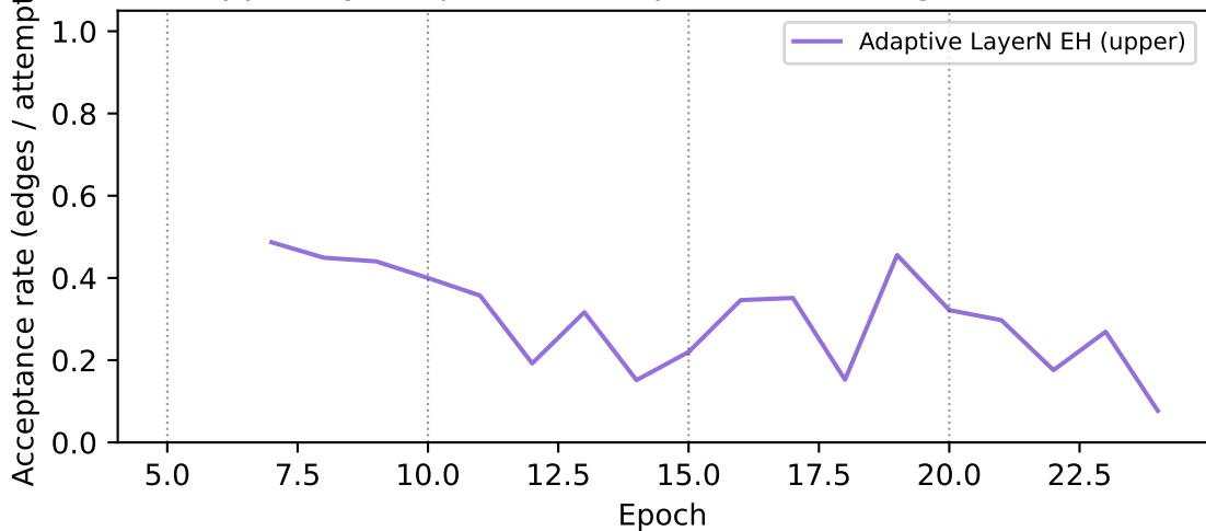
Upper-layer injection acceptance rate — gradual drift
