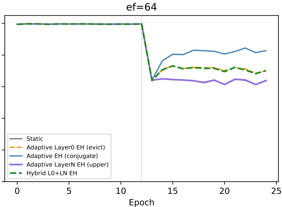
Recall@10 — sudden drift
