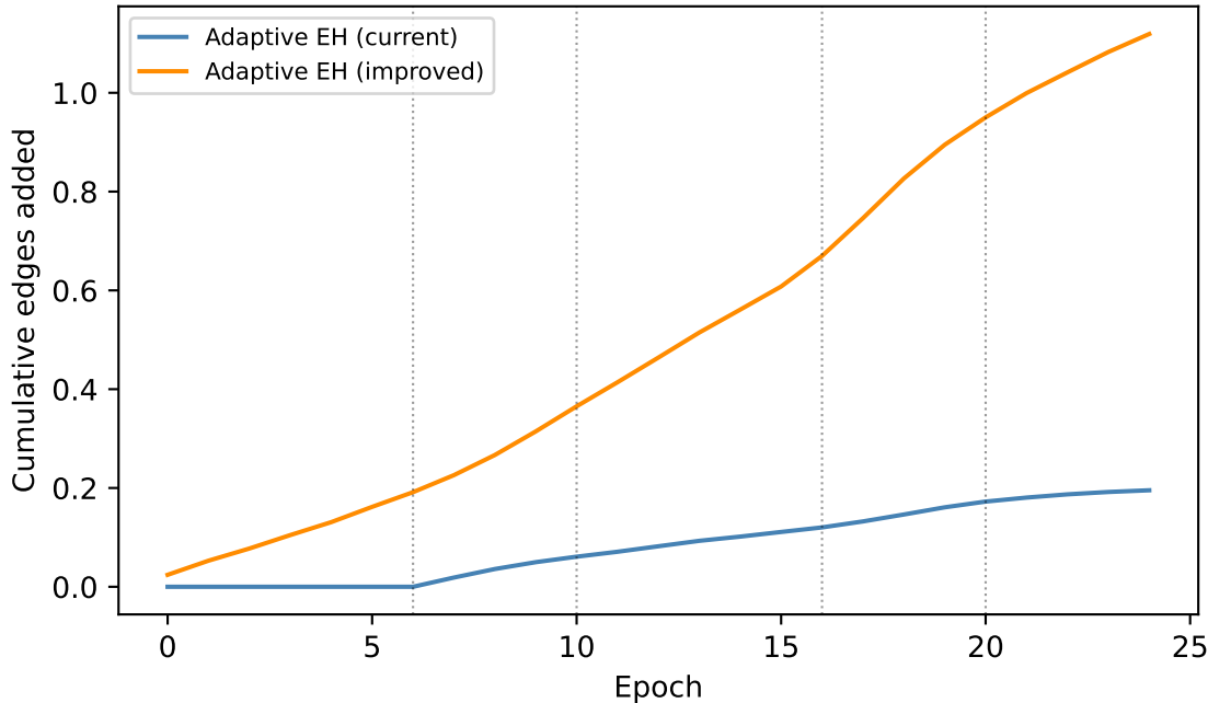
Edge count — gradual drift (SIFT rotation drift — improved adapter
