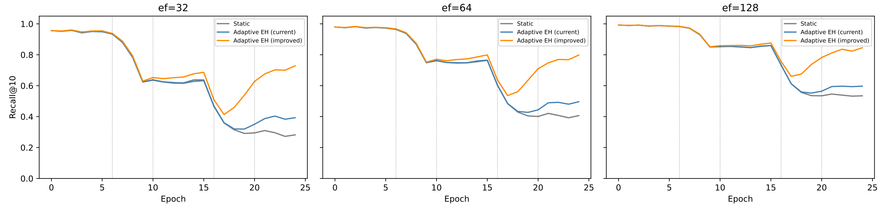
SIFT rotation drift — improved adapter (gradual)
