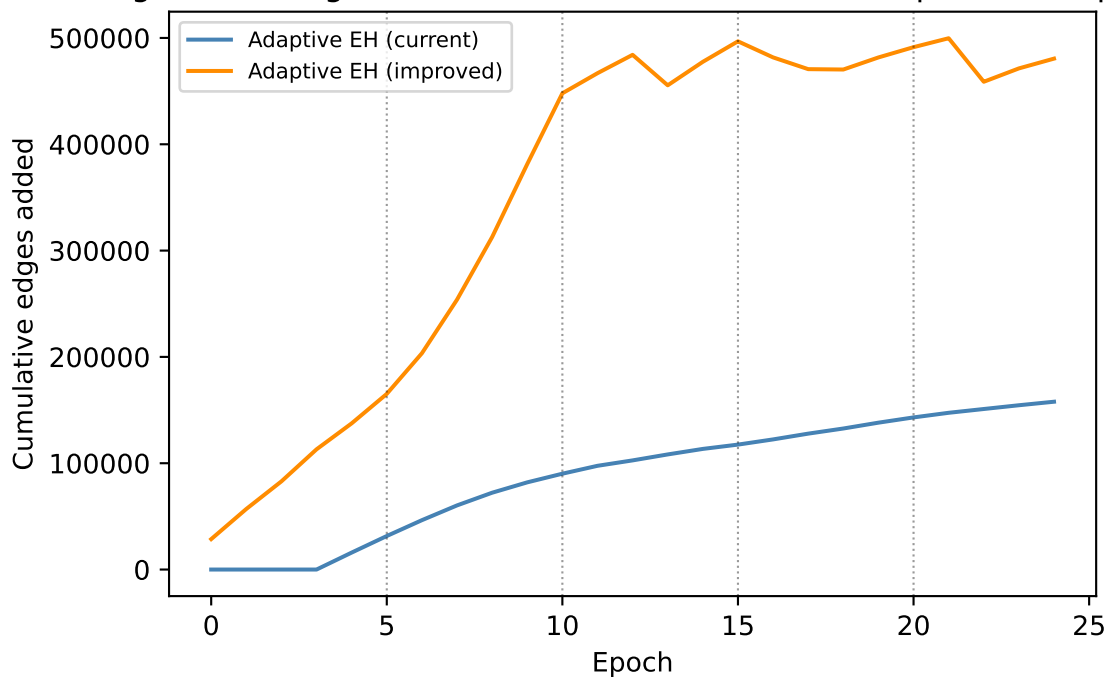
Edge count — gradual drift (SIFT rotation drift — improved adaptive
