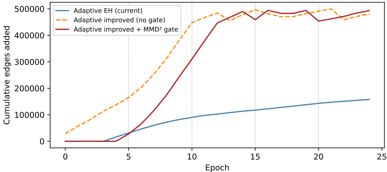
Edge count — gradual drift (mmd2gate saves pre-drift budget)
