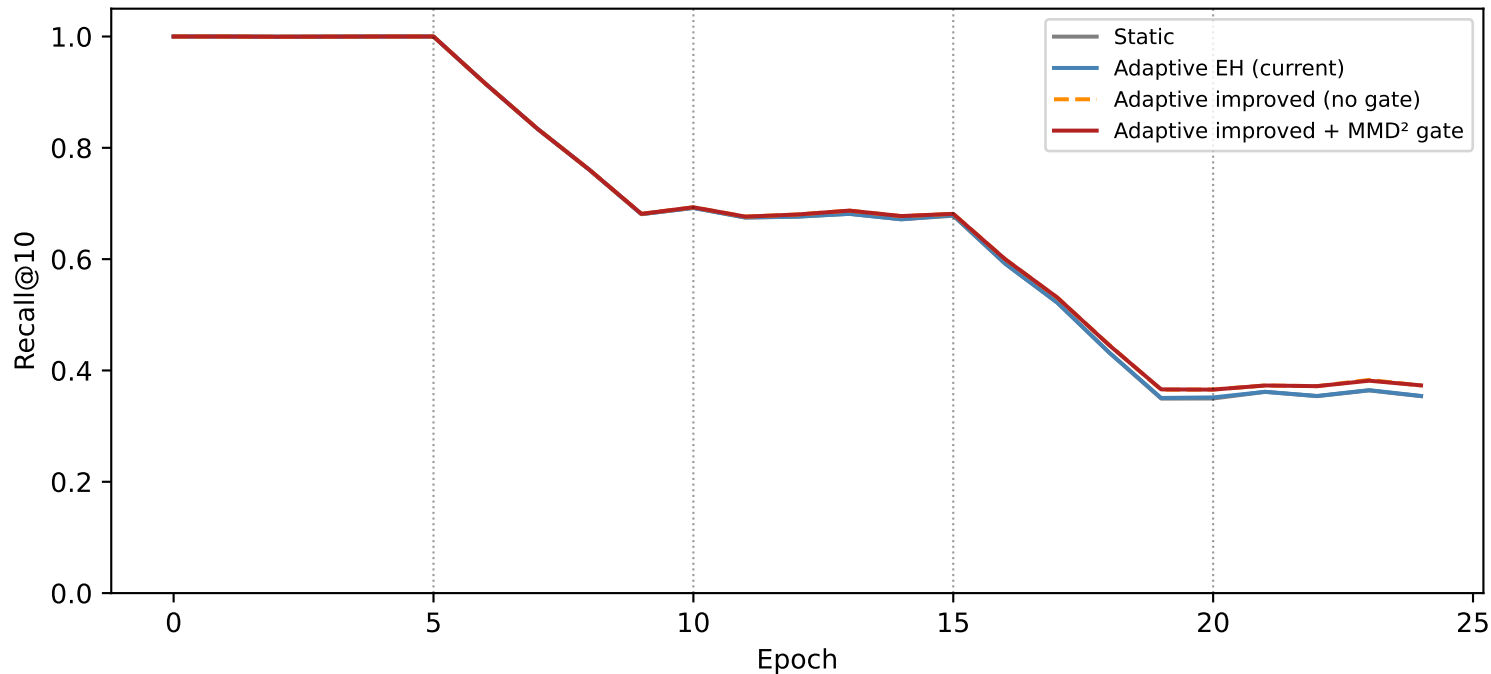
Hardness drift — MMD 2 gate comparison (gradual, ef=32)
