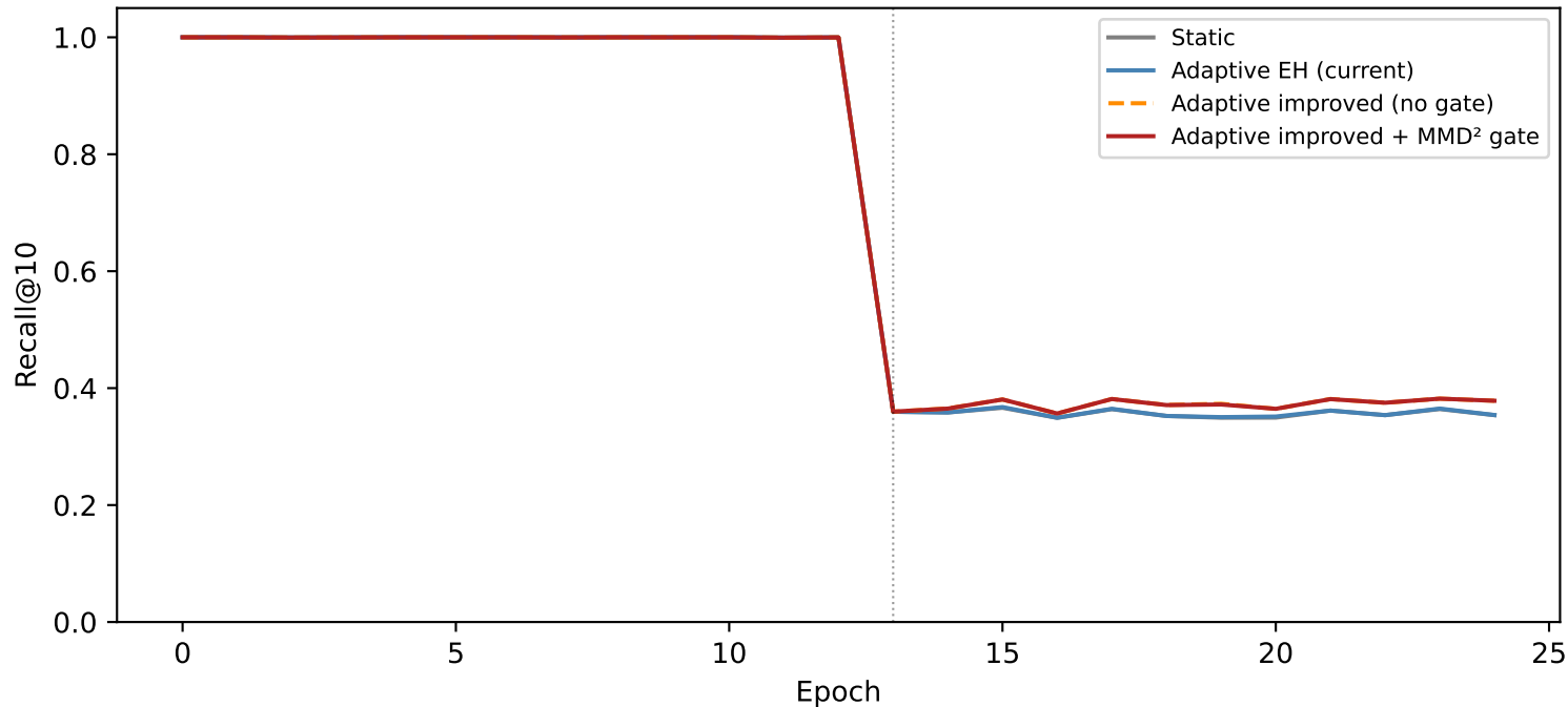
Hardness drift — MMD 2 gate comparison (sudden, ef=32)
