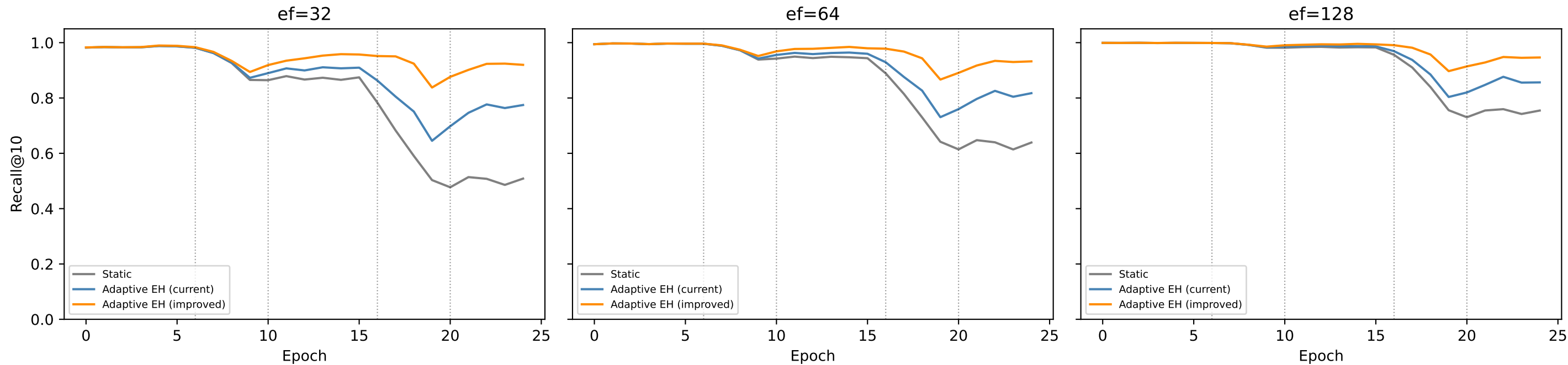
SIFT rotation drift — improved adapter (gradual)
