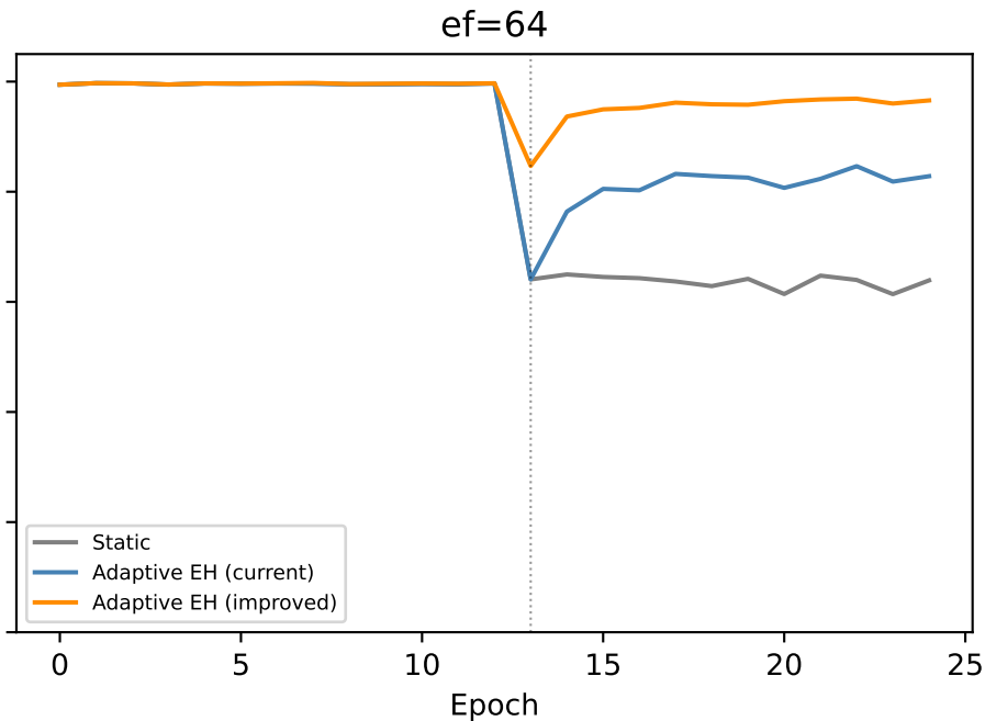
SIFT rotation drift — improved adapter (sudden)
