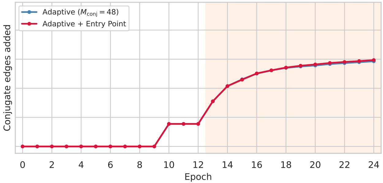
Sudden drift
