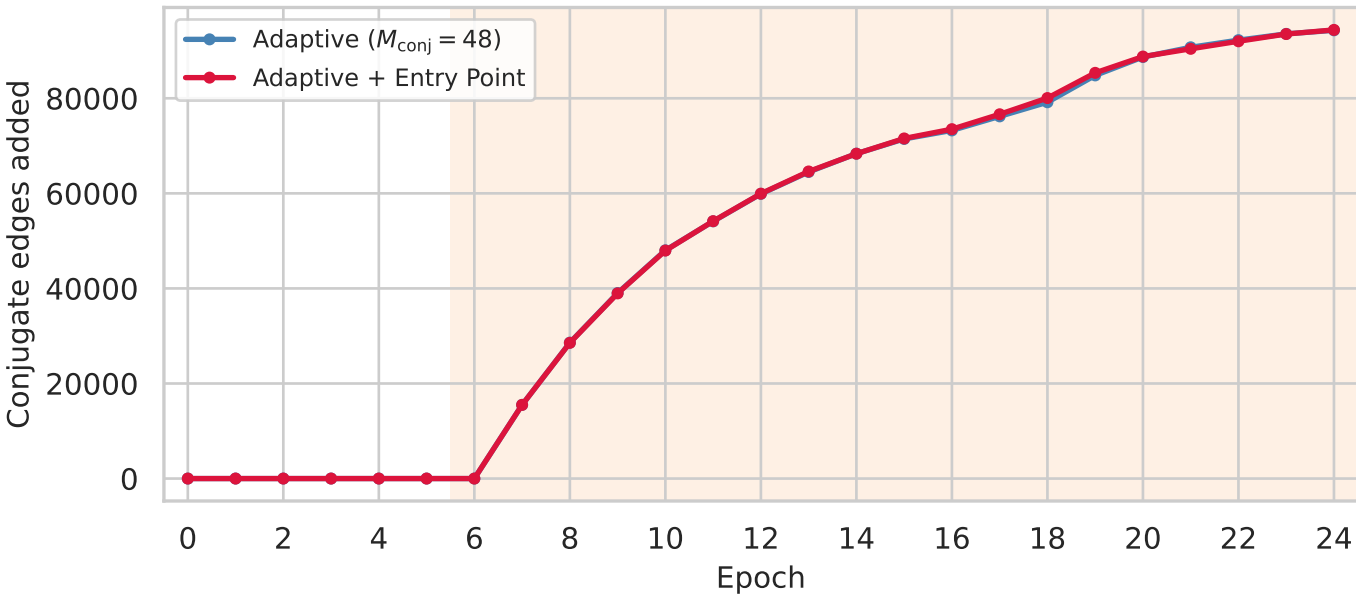
Gradual drift
