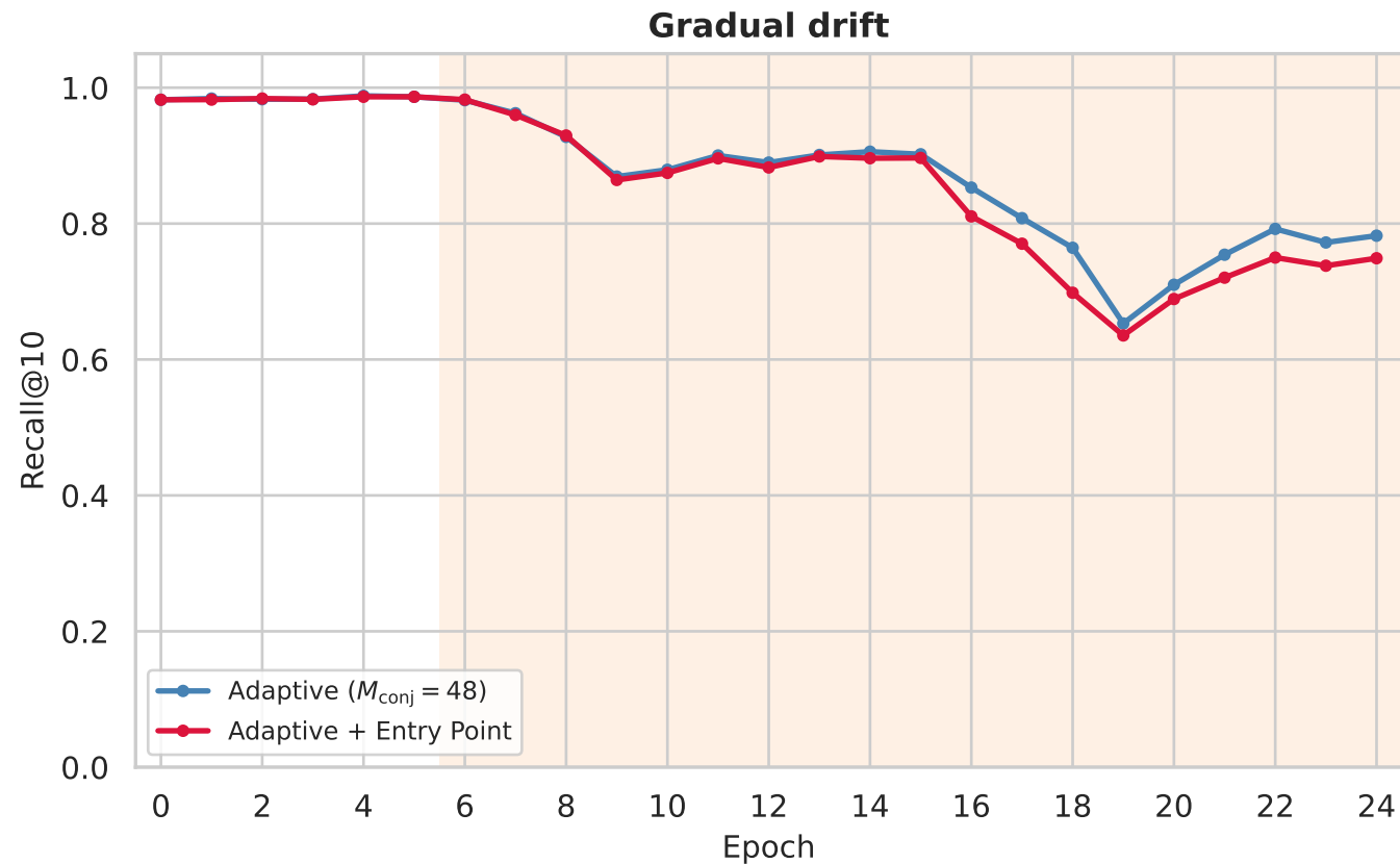
Recall@10 vs epoch — entry point adaptation (ef=32)
