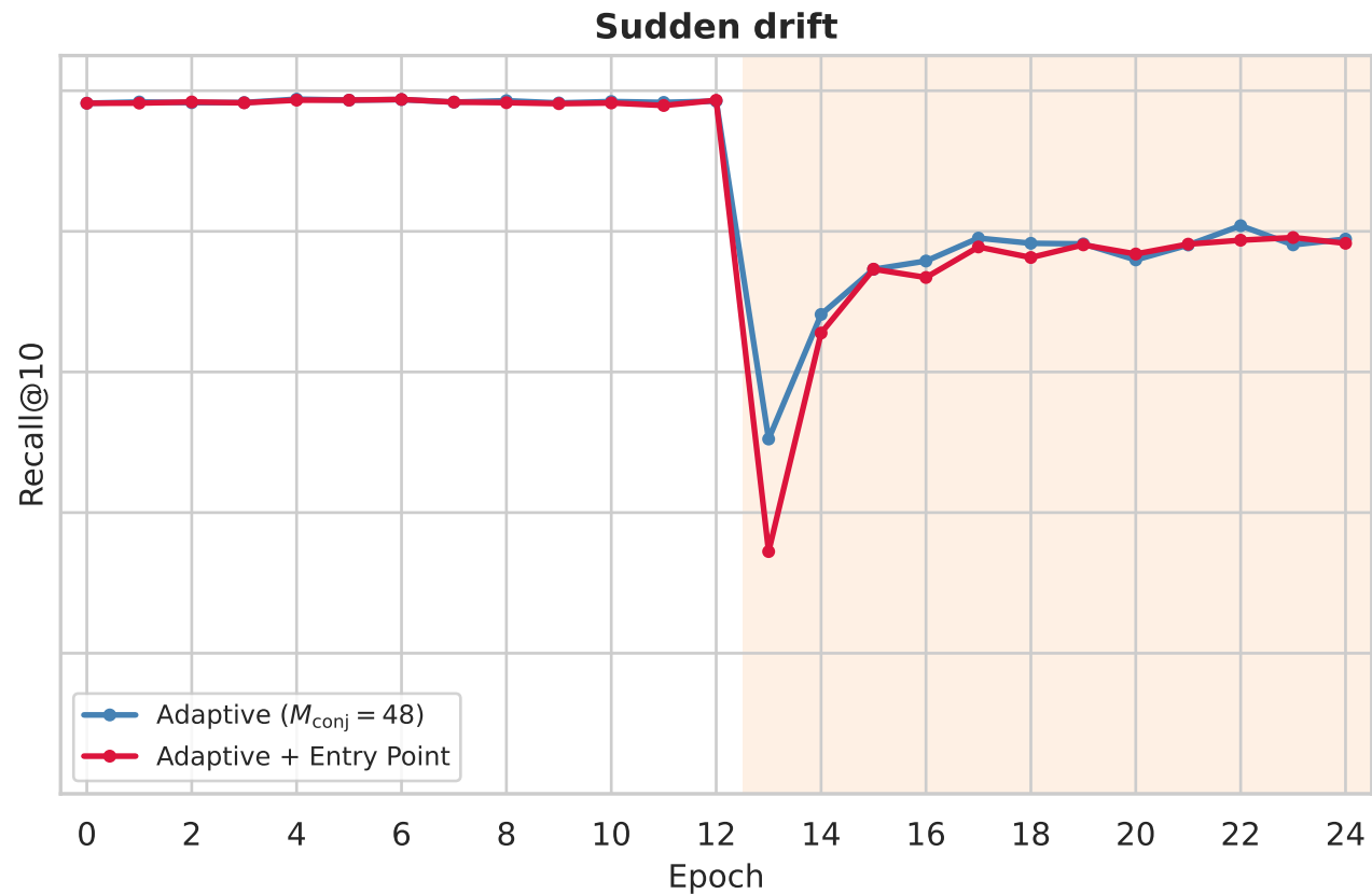
Recall@10 vs epoch — entry point adaptation (ef=32)
