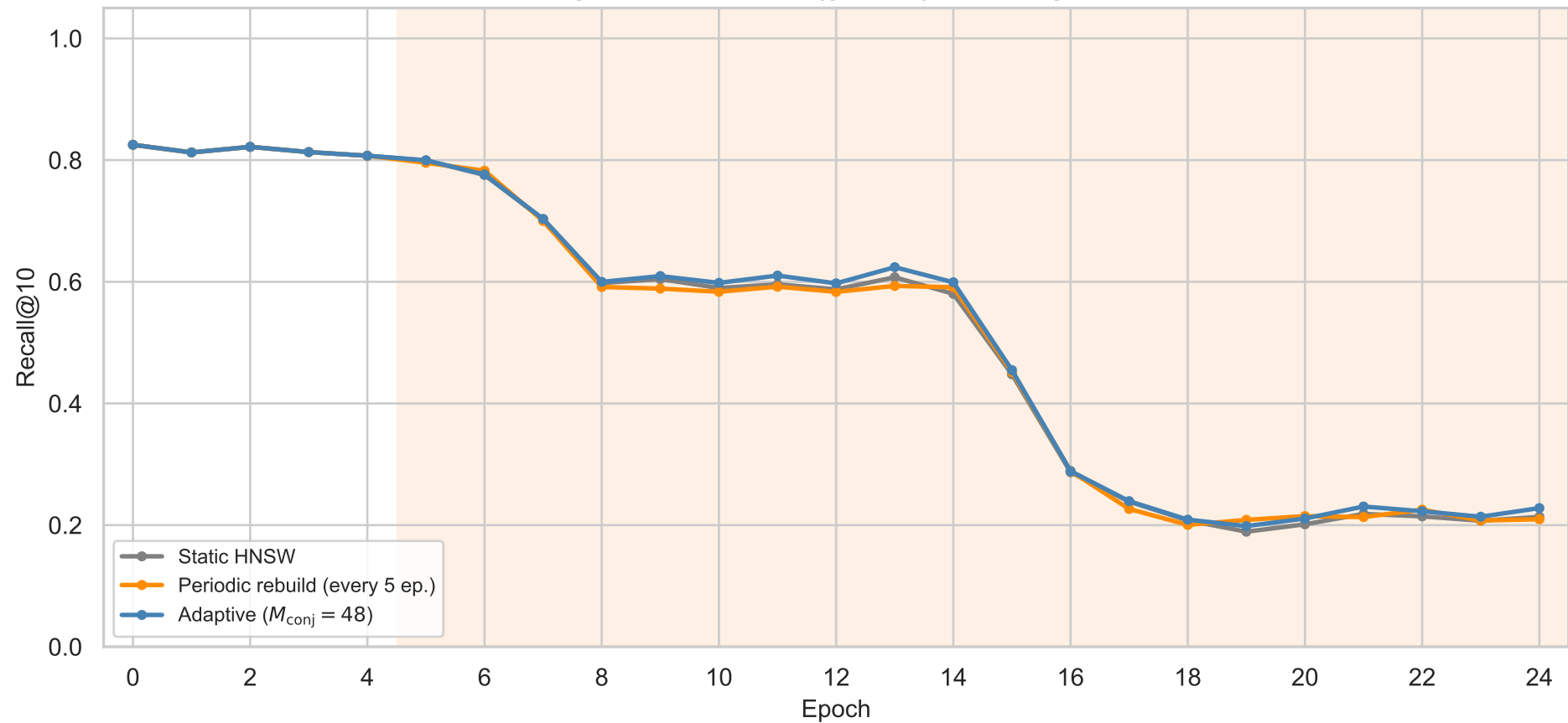
Deep-image-96 rotation drift (gradual) — recall@10 vs epoch
