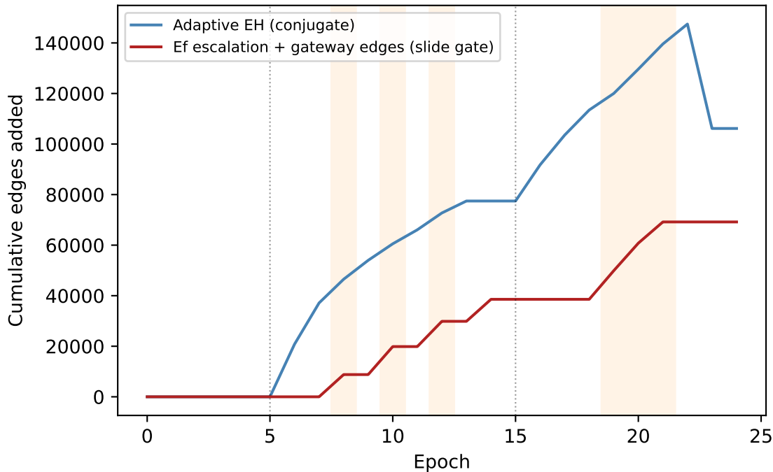
Edge count — gradual drift (DEEP-96 cluster)
