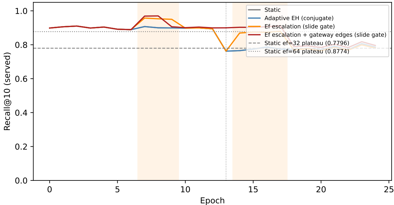
Served recall — sudden drift (what users experienced)
