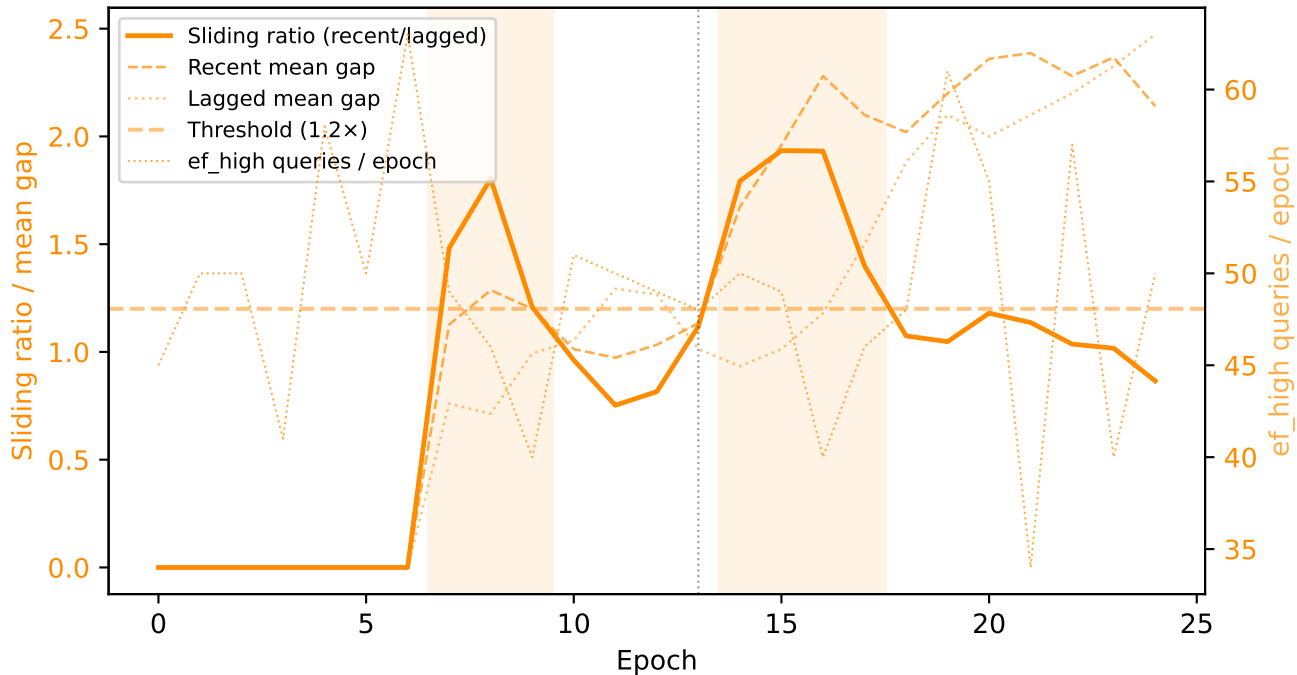
Sliding-window ratio signal and ef escalation trigger — sudden drift
