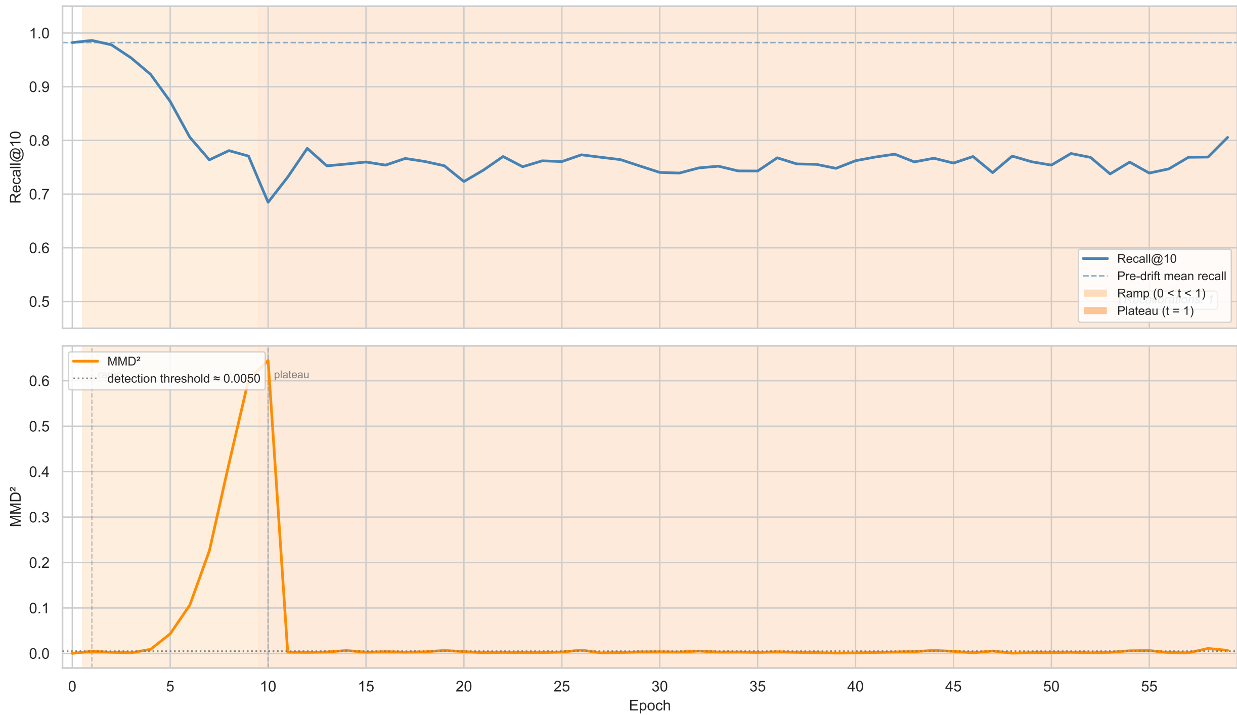
Exp 11: Recall@10 and MMD 2 over epochs — gradual drift + plateau
