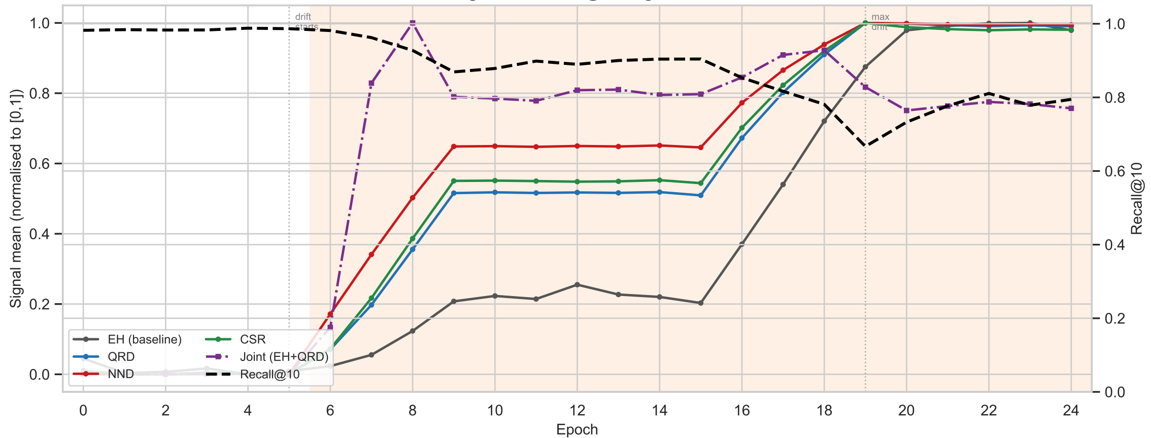
Drift signals vs. recall@10 — gradual drift
