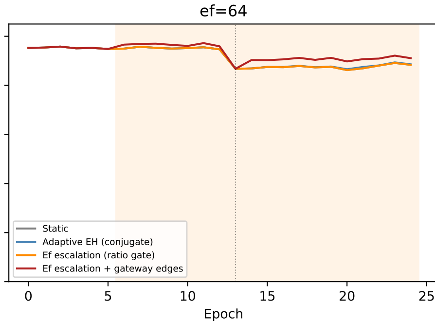
Recall@10 — sudden drift (DEEP-96 cluster, exp50)
