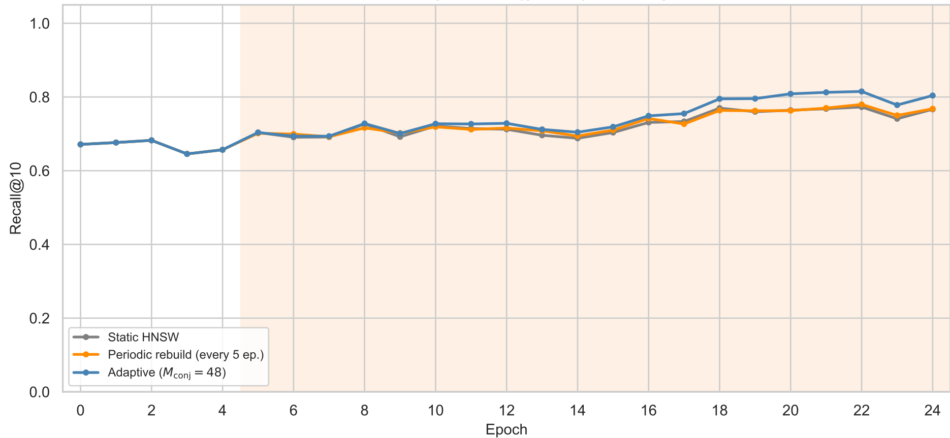
GloVe-100 cluster-reweighted drift (gradual) — recall@10 vs epoch
