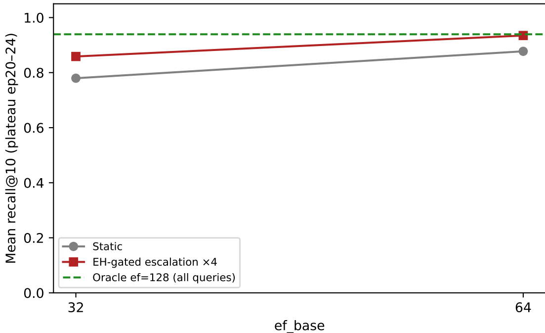
ef-scaling at plateau — sudden drift
