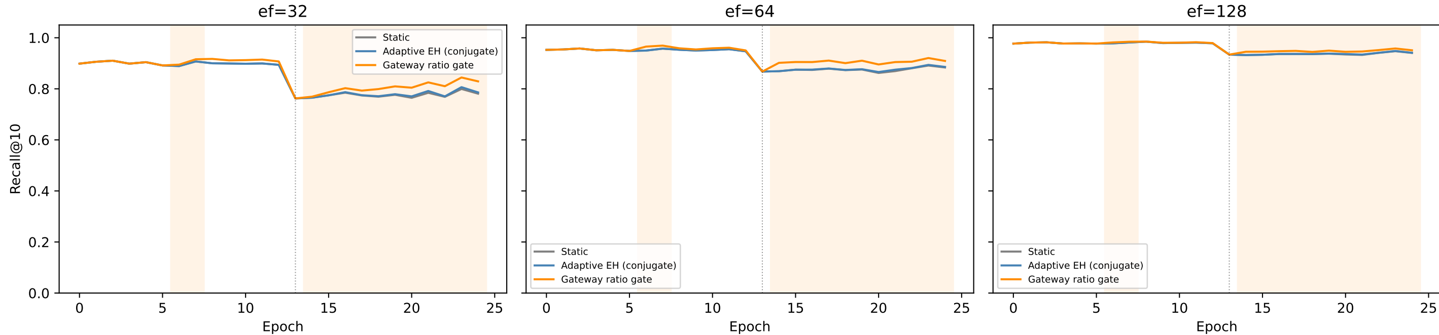
Recall@10 — sudden drift (DEEP-96 cluster, exp49)
