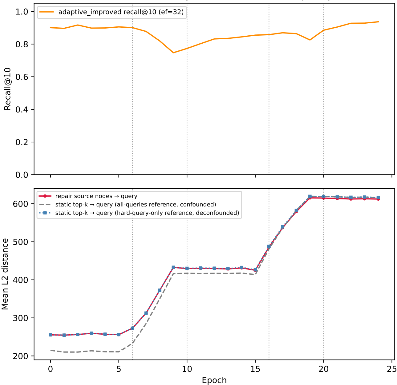
SIFT1M rotation drift — gradual — feedback-loop diagnostic
