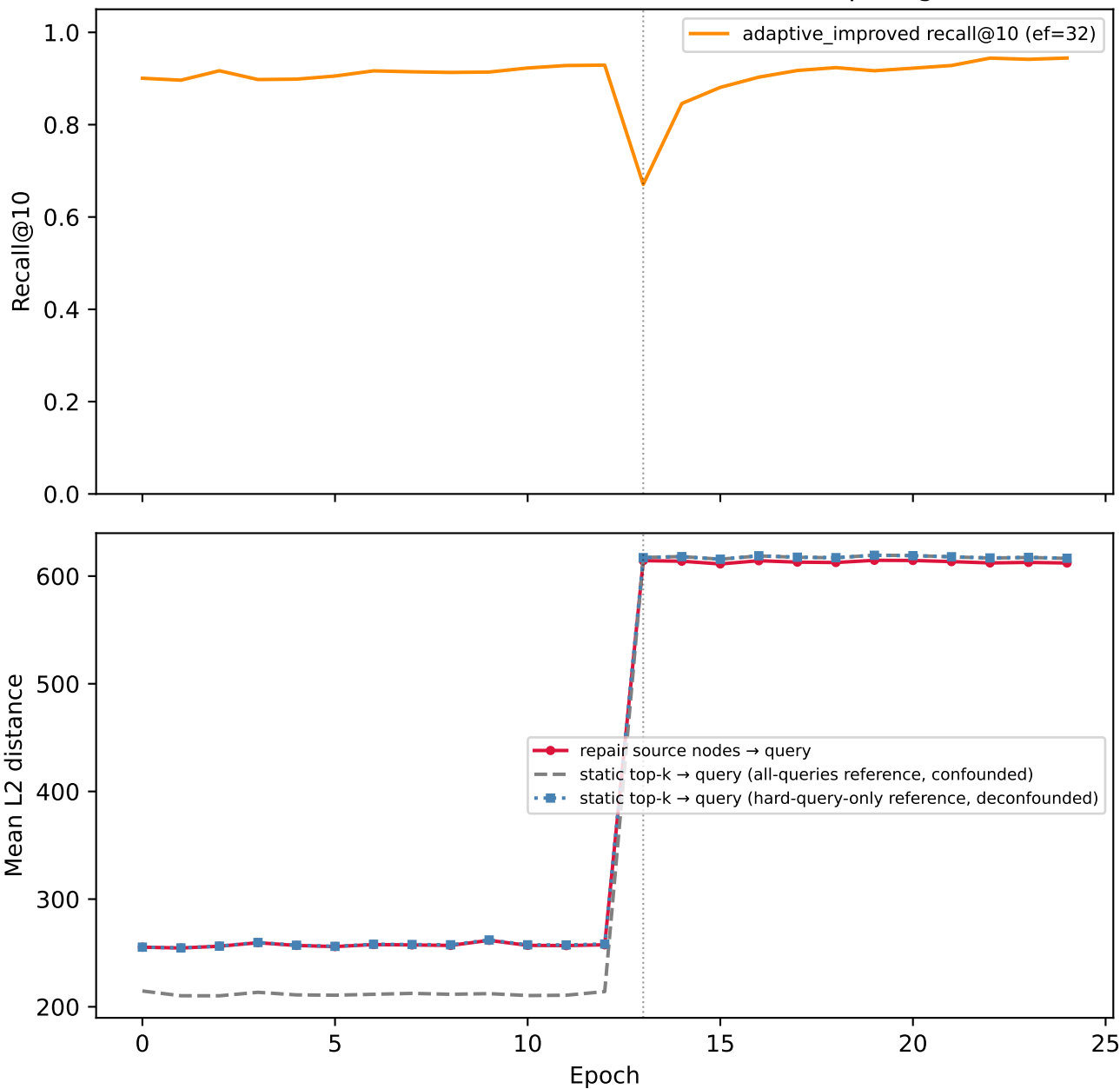
SIFT1M rotation drift — sudden — feedback-loop diagnostic
