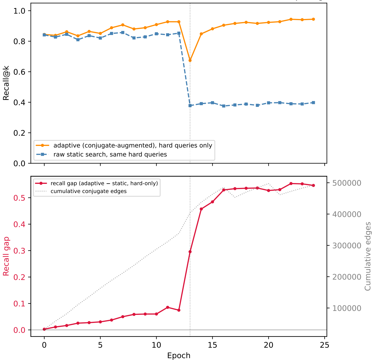
SIFT1M rotation drift — sudden — matched-recall feedback-loop diagnostic
