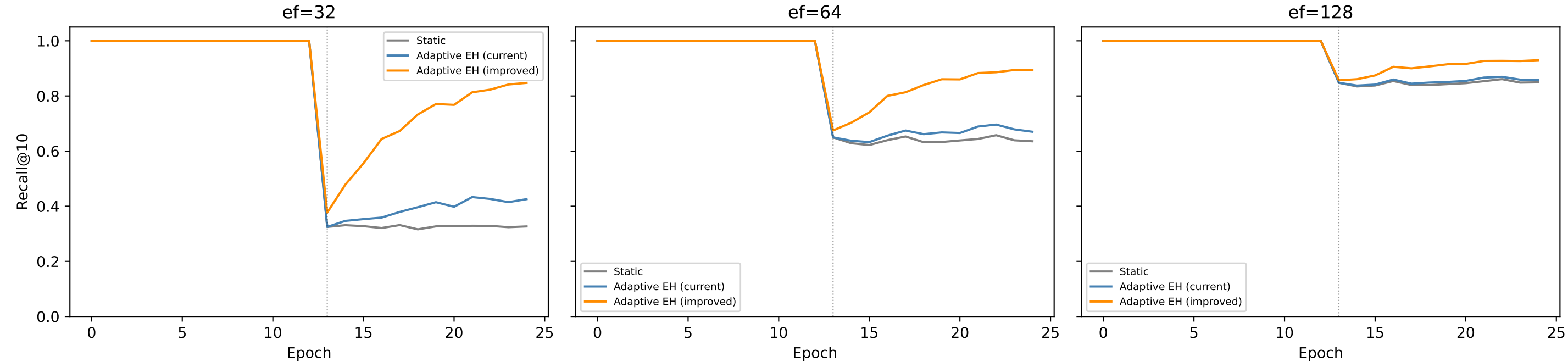
Clustered structural hardness drift — improved adapter (sudden)
