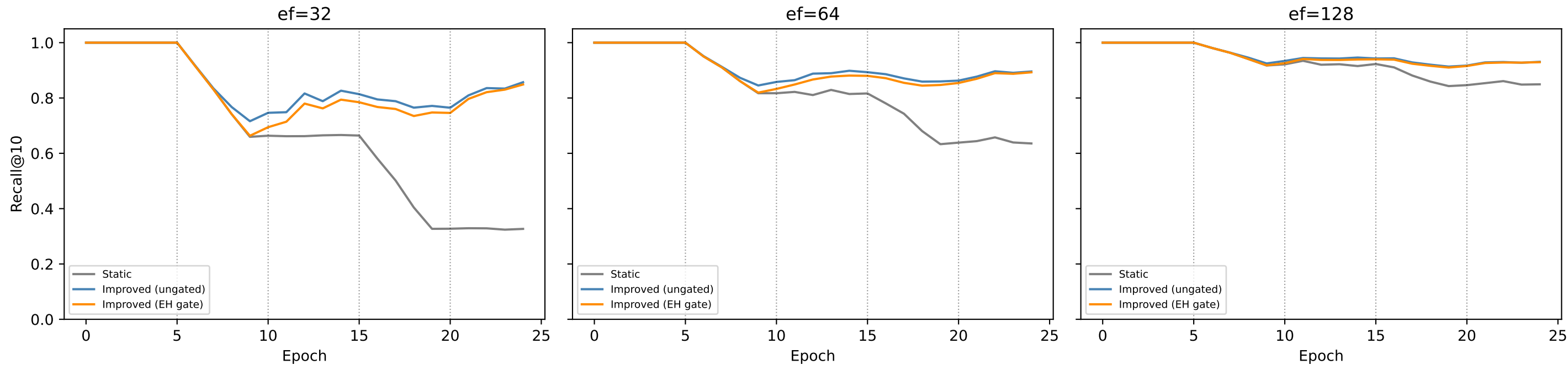
Clustered hardness drift — population EH gate (gradual)
