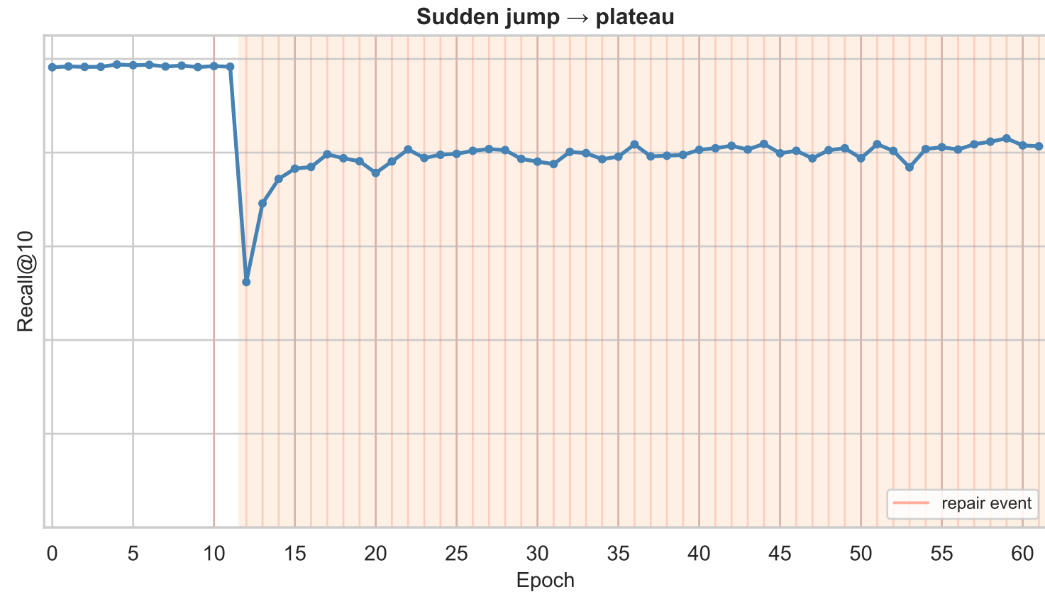
Recall@10 vs epoch (ef=32, M_conj=48)
