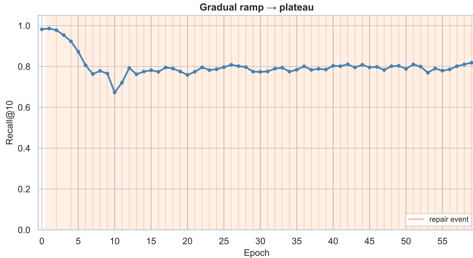
Recall@10 vs epoch (ef=32, M_conj=48)
