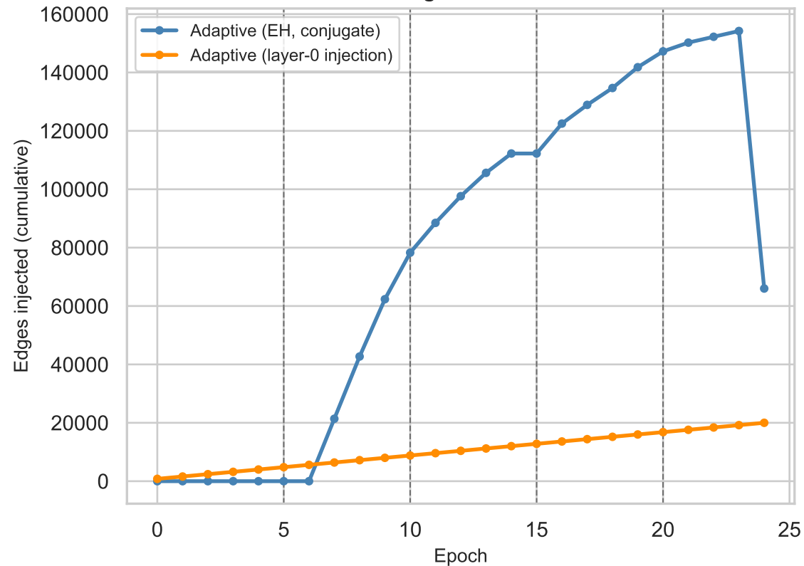
gradual
