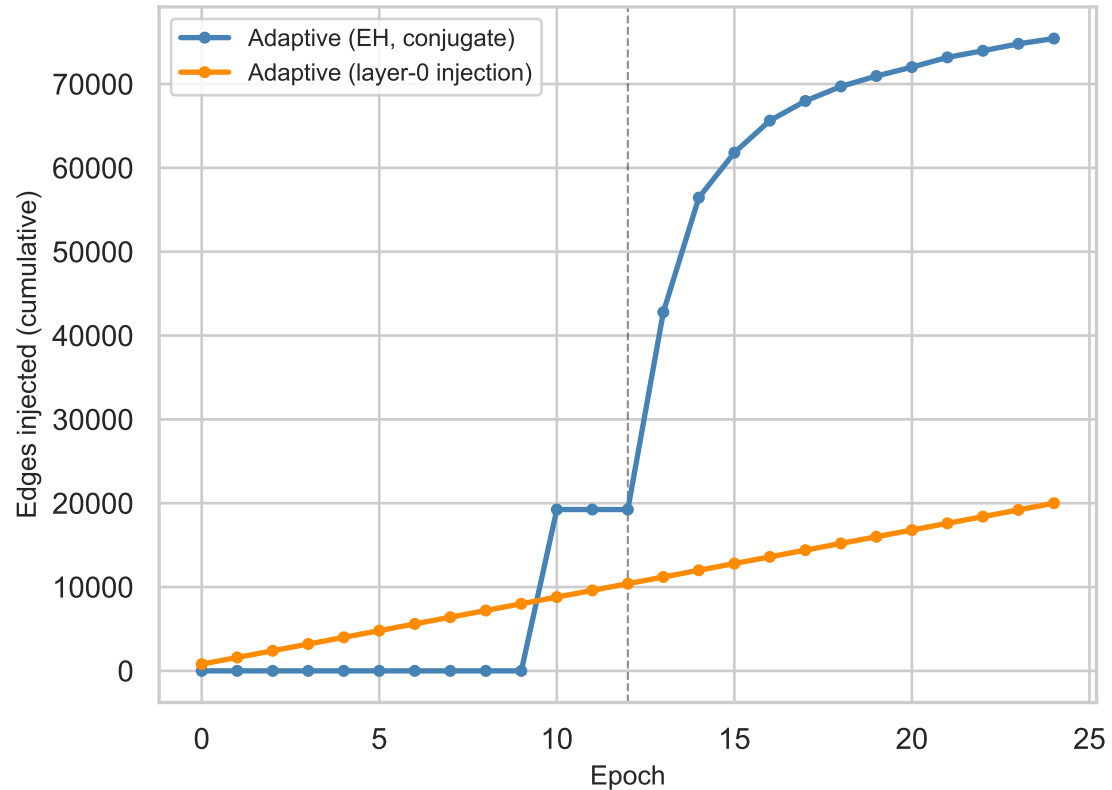
sudden
