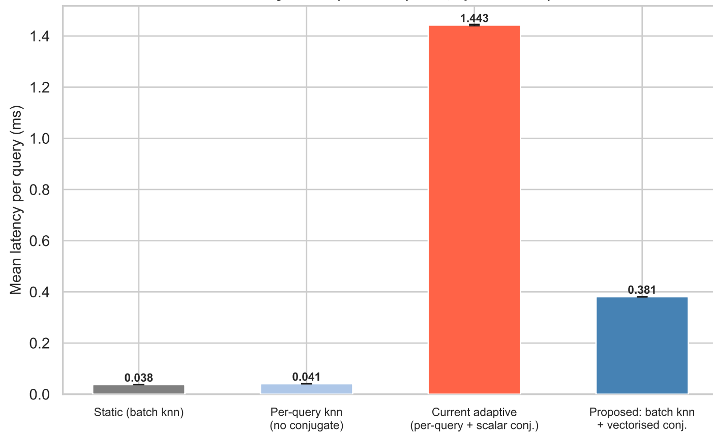
Latency decomposition (ef=32, epoch-24 CG)
