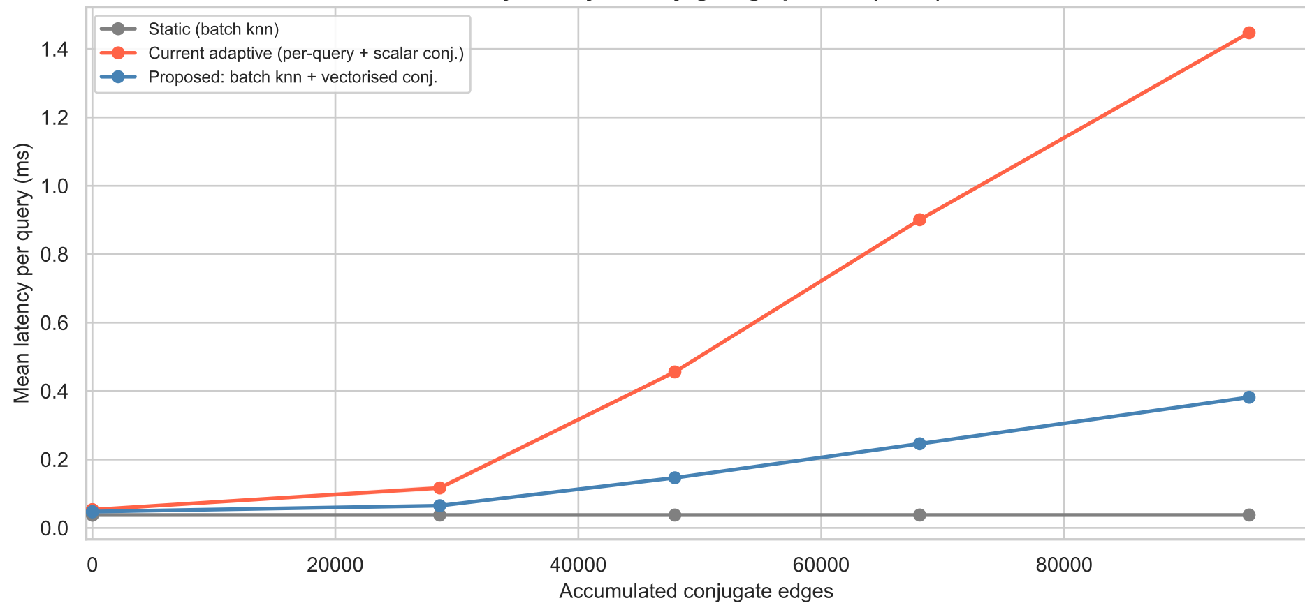
Query latency vs conjugate graph size (ef=32)
