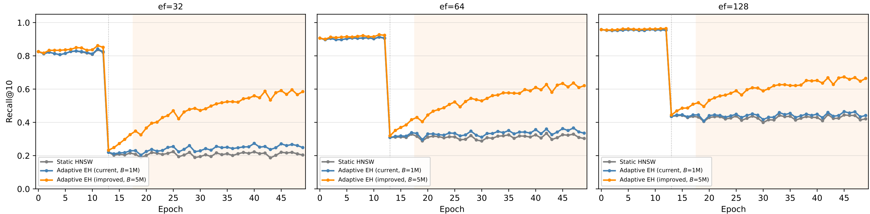
DEEP-96 rotation drift (Sudden) — Recall@10 vs Epoch
