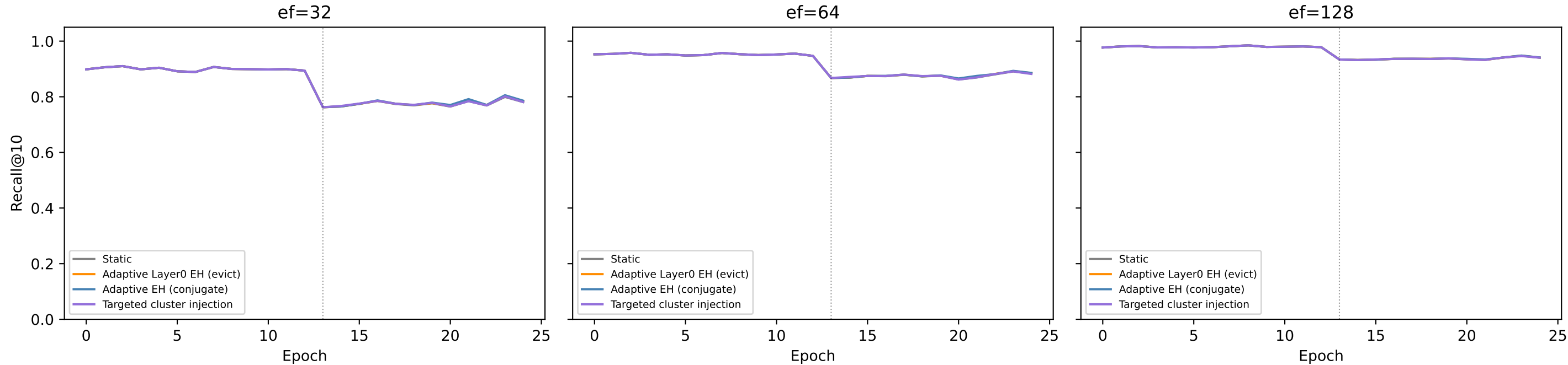
Recall@10 — sudden drift (DEEP-96 cluster)
