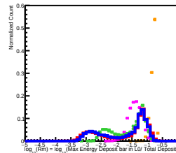
100 GeV incident in L4
