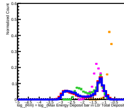
50 GeV incident in L3
