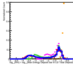
600 GeV incident in L4
