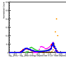
600 GeV incident in L3
